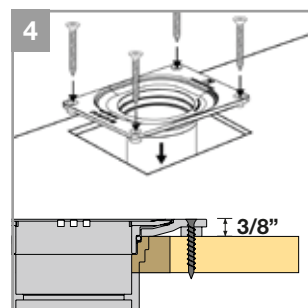
4. Screw the drainbody to the substrate and check the height 3/8". View heights in page 19. In concrete installations set the drain levelled with thinset.
