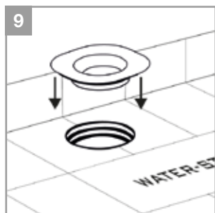
9. Place the bonding flange in top of the drainbody and press until it is lush and locked.
