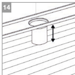
14. Adjust the height of the drain depending on the tile thickness.
