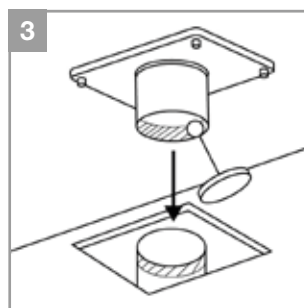
3. Verify the drainpipe is at least at 1-3/8" (33 mm) of the substrate surface. Glue the drain body to the drainpipe using the proper adhesive (ABS – black or PVC – white).
