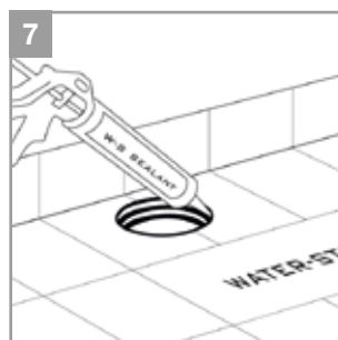
7. Lift the edge of the WATER-STOP sheet, insert the cannula of the W-S Sealant 1/2" and apply a continuous line of mastic in the connection drainbody – WATER-STOP.
