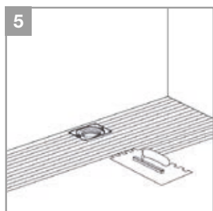
5. Apply thin set cement in the drain shower area with a 1/4" notched trowel from the shower perimeter to the drain. RECOMMENDED THINSET ANSI A118.4, ANSI A118.11 and ANSI A118.15.
