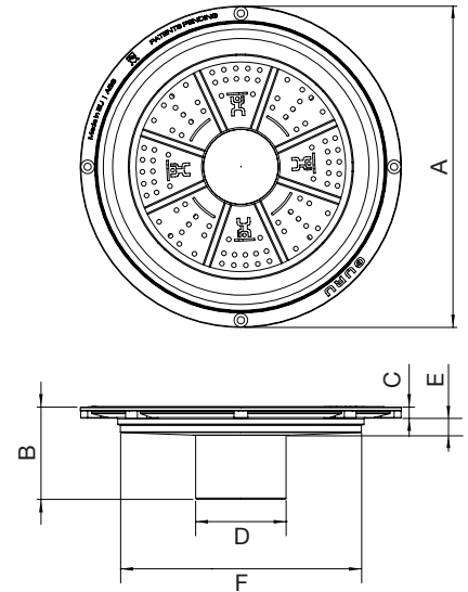
DRAIN MEASUREMENTS
