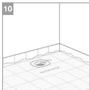
10. Flood test according to local code. If W-S Sealant has been used to install the corners, the test can be performed after 1 hour.
